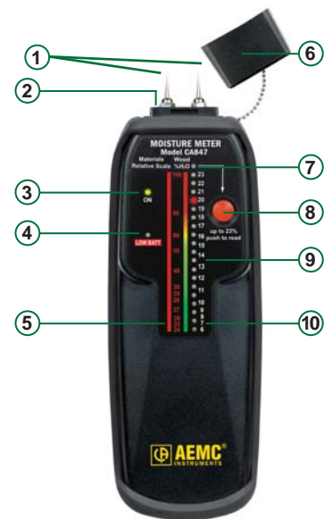
Protective cover also acts as power switch – remove cover to turn instrument on; replace cover to turn instrument off.
